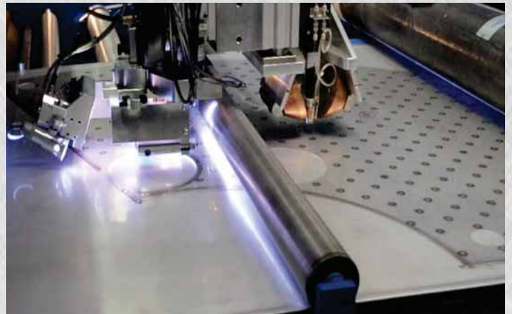
APPLYING PROTECTION FILM
